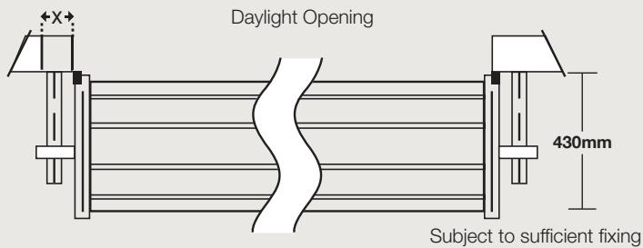
Plan View
