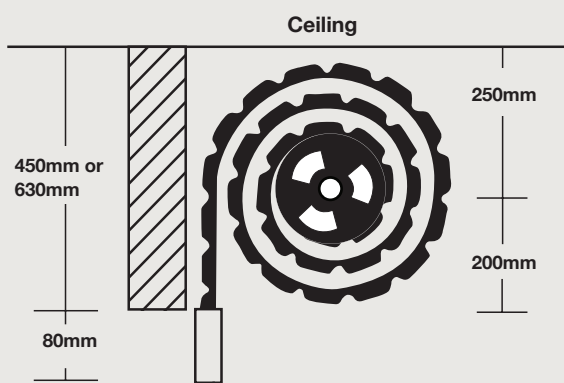
End View
