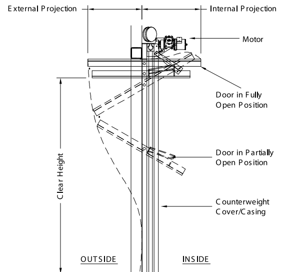
SECTION VIEW
